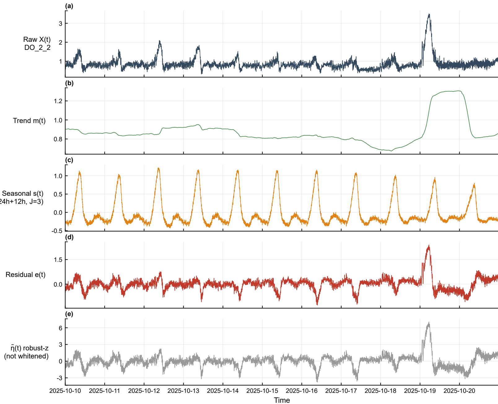
Multi-scale decomposition — DO_2_2 (aerobic, min) [2025-10-10~2025-10-20]
